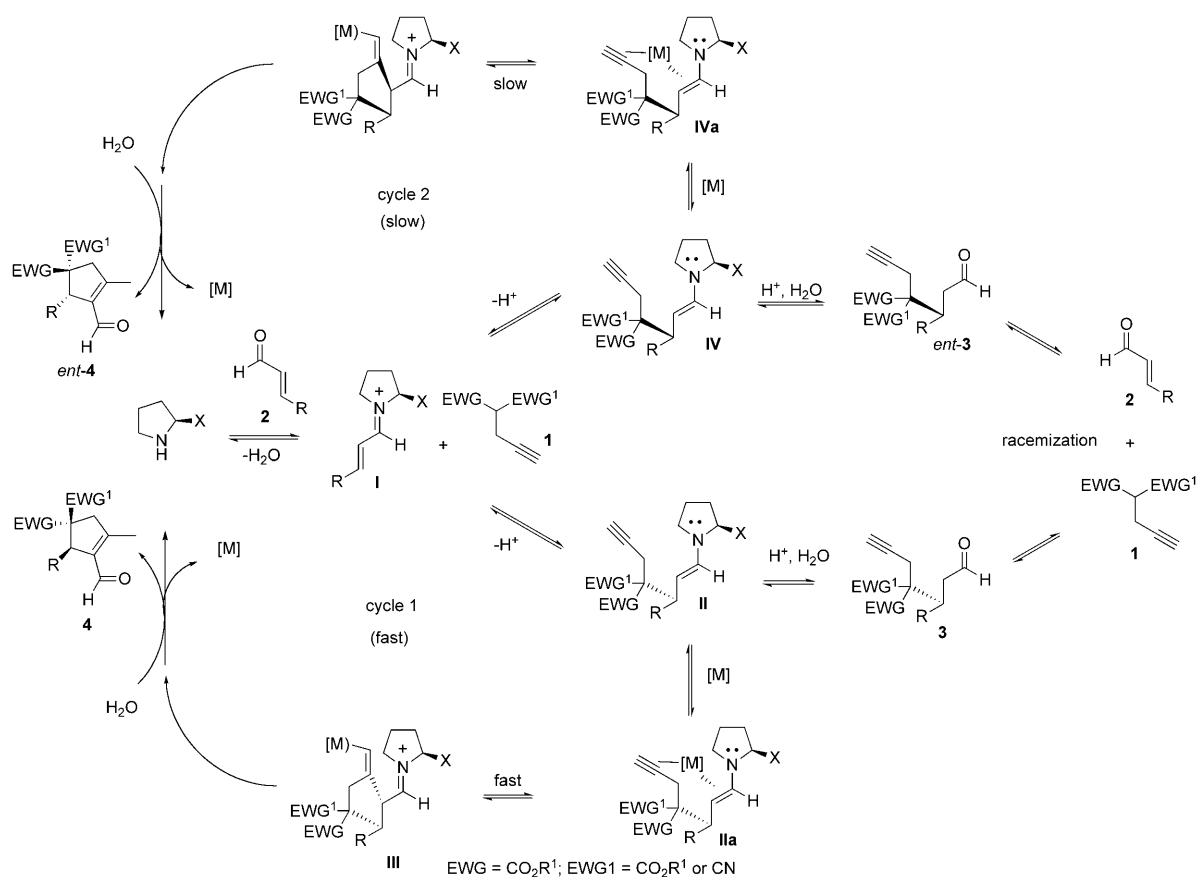
Scheme 1. Combined transition-metal- and amine-catalyzed DYKAT.
